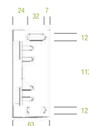
supporto parete / soffitto wall / ceiling fixing bracket
