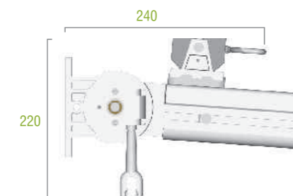
supporto parete / soffitto con guida wall / ceiling fixing bracket with rail
